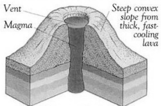
Dome volcano
