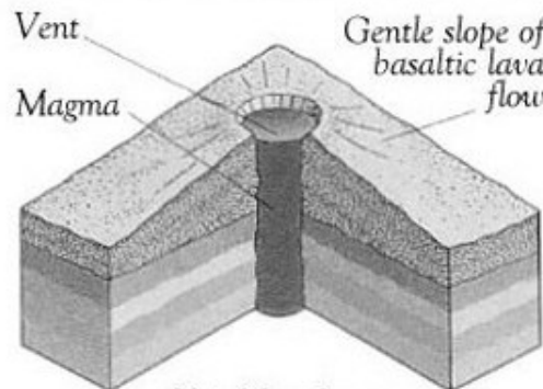
Shield volcano
