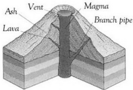
Composite volcano
